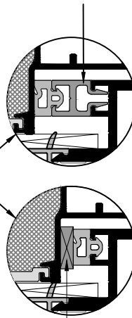
For 32mm glazing 4mm packer required
