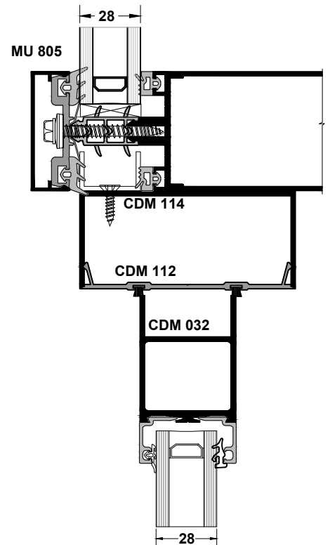
Commercial door into curtain wall
